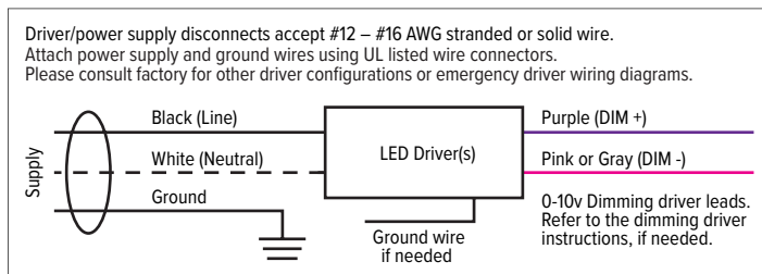
FIGURE 12.1 Make electrical connections in accordance with NEC and local codes.
