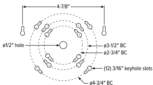
WALL MOUNT BOLT CIRCLE PATTERN
