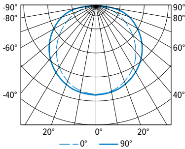
FT-24-LS/8CS-AF-DIM-UNV Total Luminaire Output: 4111 lumens; 27.3 Watts (Low Wattage Setting) | Efficacy: 151 lm/W | 80 CRI; 3500K CCT
