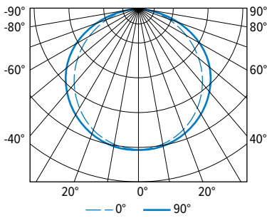
FT-22-LS/8CS-AF-DIM-UNV Total Luminaire Output: 2534 lumens; 17.5 Watts (Low Wattage Setting) | Efficacy: 145 lm/W | 80 CRI; 3500K CCT
