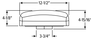
Straight Arm Front view EPA: 1.00/Weight: 20 Lbs.
