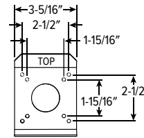
Mounting plate
